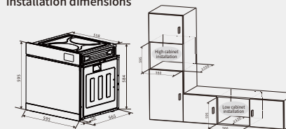
Installation dimensions
