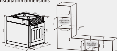
Installation dimensions
